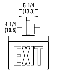
With Pendant Mounting kit (TM mounting only)
