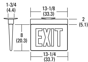
Top Mount (AC only operation)
